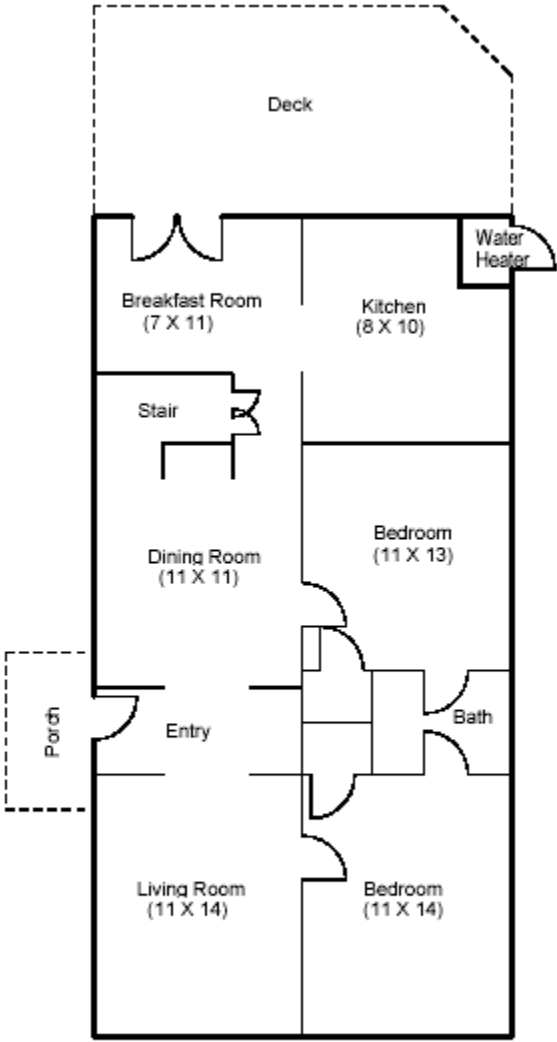
Main Level
